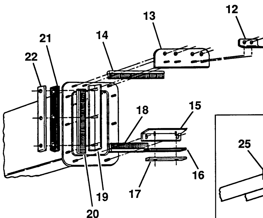
Detail . . . Mid Boom Wiper Arrangement
