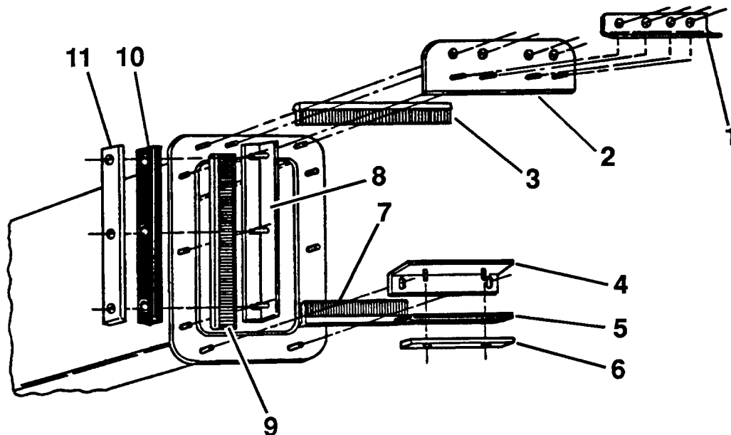
Detail . . . Base Boom Wiper Arrangement
