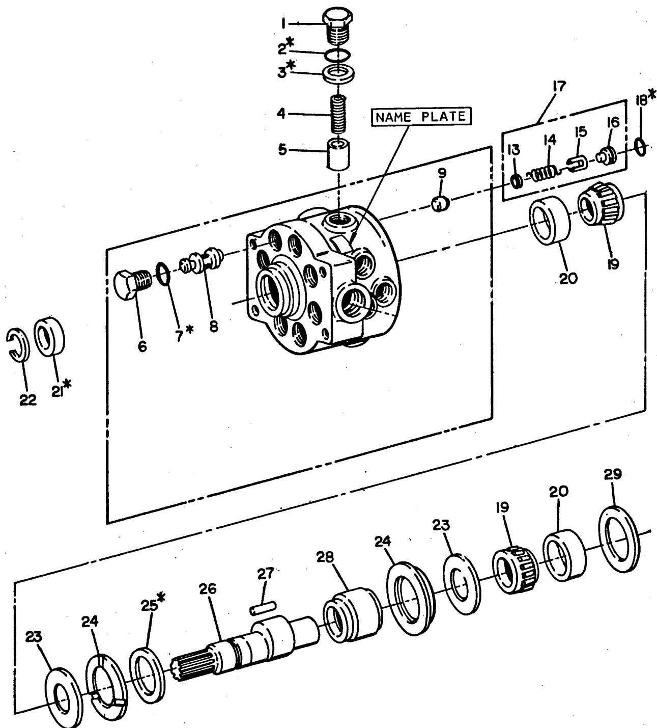
PUMP ASSEMBLY
